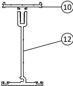
E9-4652 VERTICAL MULLION
