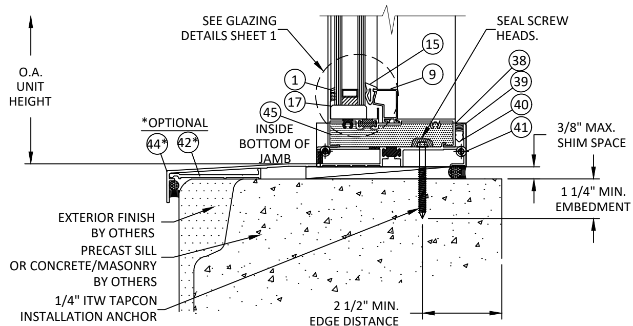
H 6 VERTICAL SECTION SILL - CONCRETE/MASONRY THROUGH FRAME
