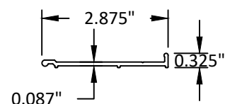
42 SILL TRIM BASE 6063-T5
