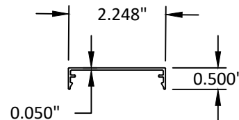
11 FACE COVER 6063-T5
