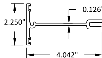
12 STACKING MULLION 6063-T5
