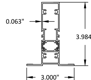
37 INTEGRAL MULLION 6063-T5
