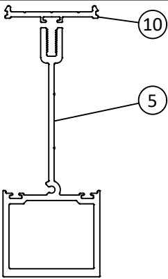
E9-4753 VERTICAL MULLION
