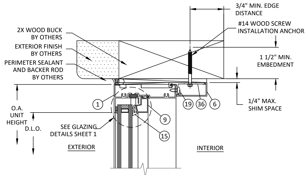
F 6 VERTICAL SECTION HEAD - 2X WOOD BUCK CLIP ANCHOR
