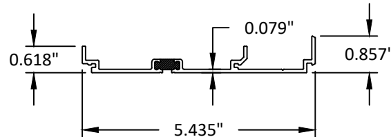
7 STRAP ANCHOR 6063-T5
