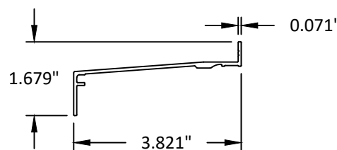
43 3" SILL TRIM 6063-T5
