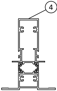
BE9-5703 HORIZONTAL MULLION
