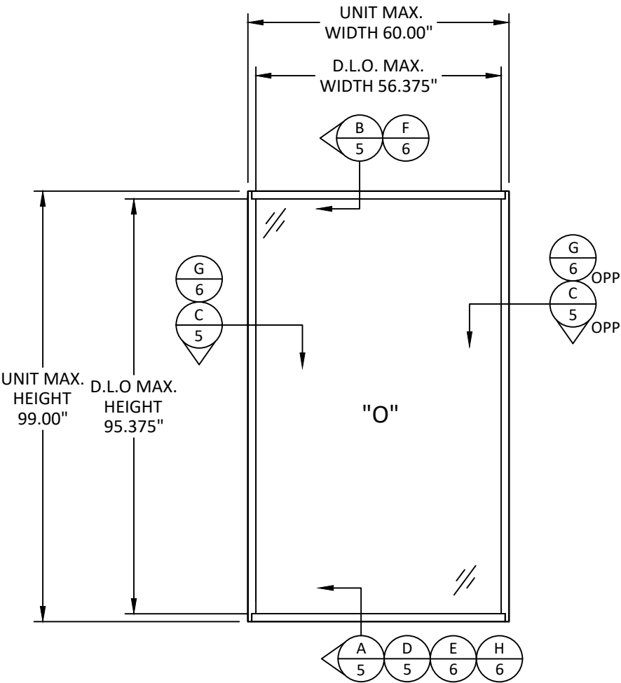
ELEVATION TYPICAL
