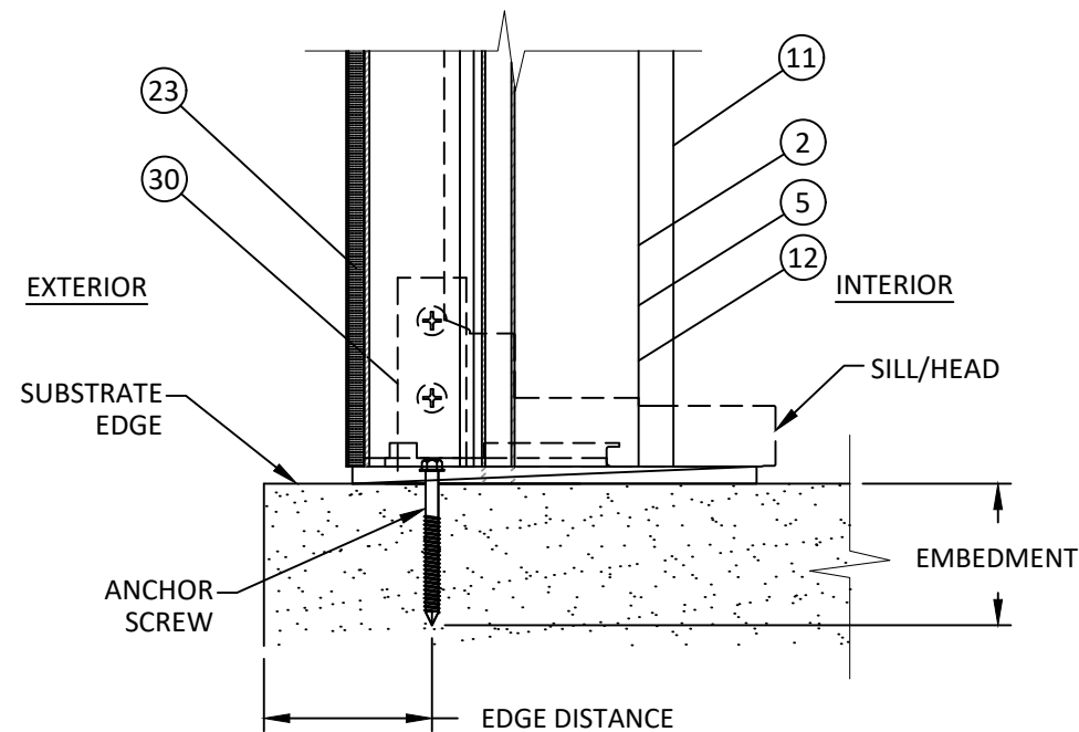
M 8 MULLION TRANSVERSAL SECTION
