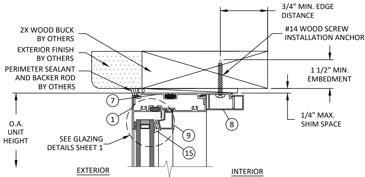
B 5 VERTICAL SECTION HEAD - 2X WOOD BUCK STRAP ANCHOR
