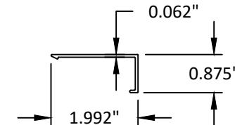
6 7/8" x 2" CLIP ANCHOR COVER 6063-T5
