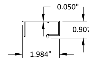
8 STRAP ANCHOR COVER 6063-T5
