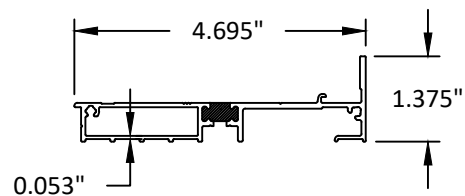
39 4" WEEPING SILL FLASHING 6063-T5
