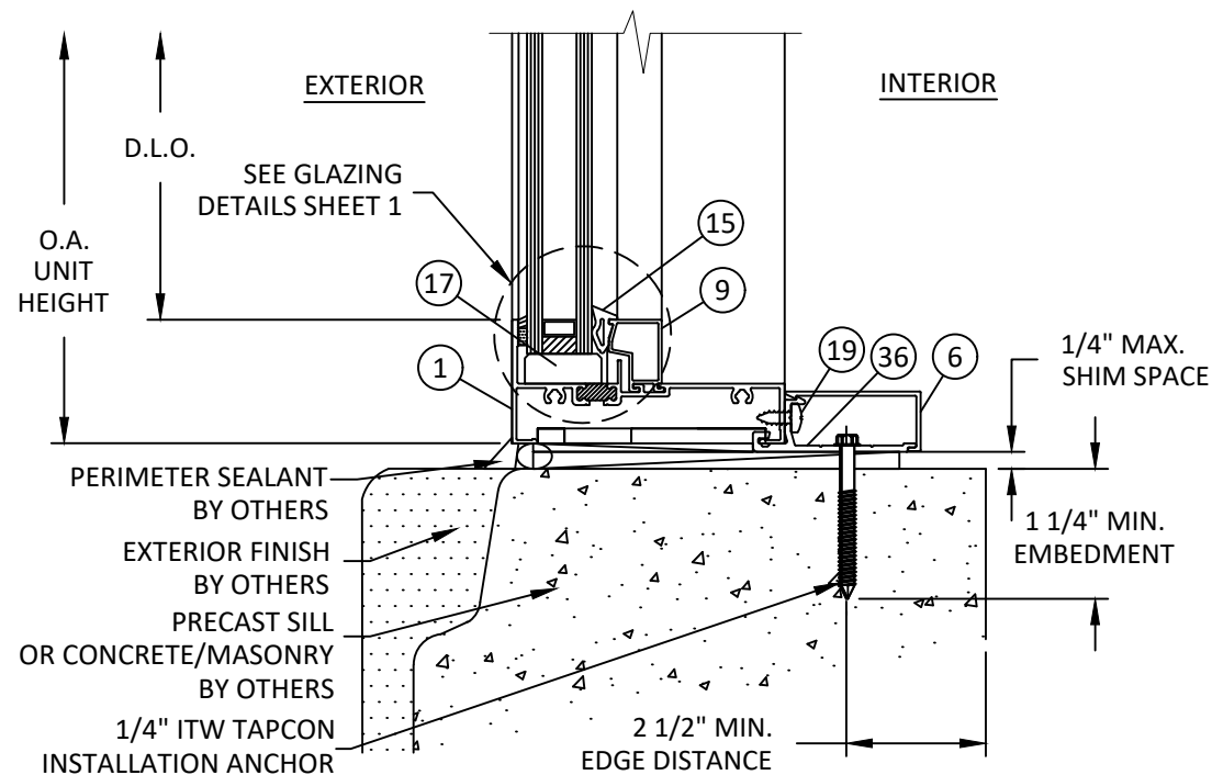
E 6 VERTICAL SECTION SILL - CONCRETE/MASONRY CLIP ANCHOR
