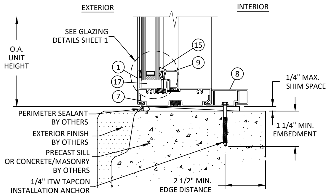
A 5 VERTICAL SECTION SILL - CONCRETE/MASONRY STRAP ANCHOR
